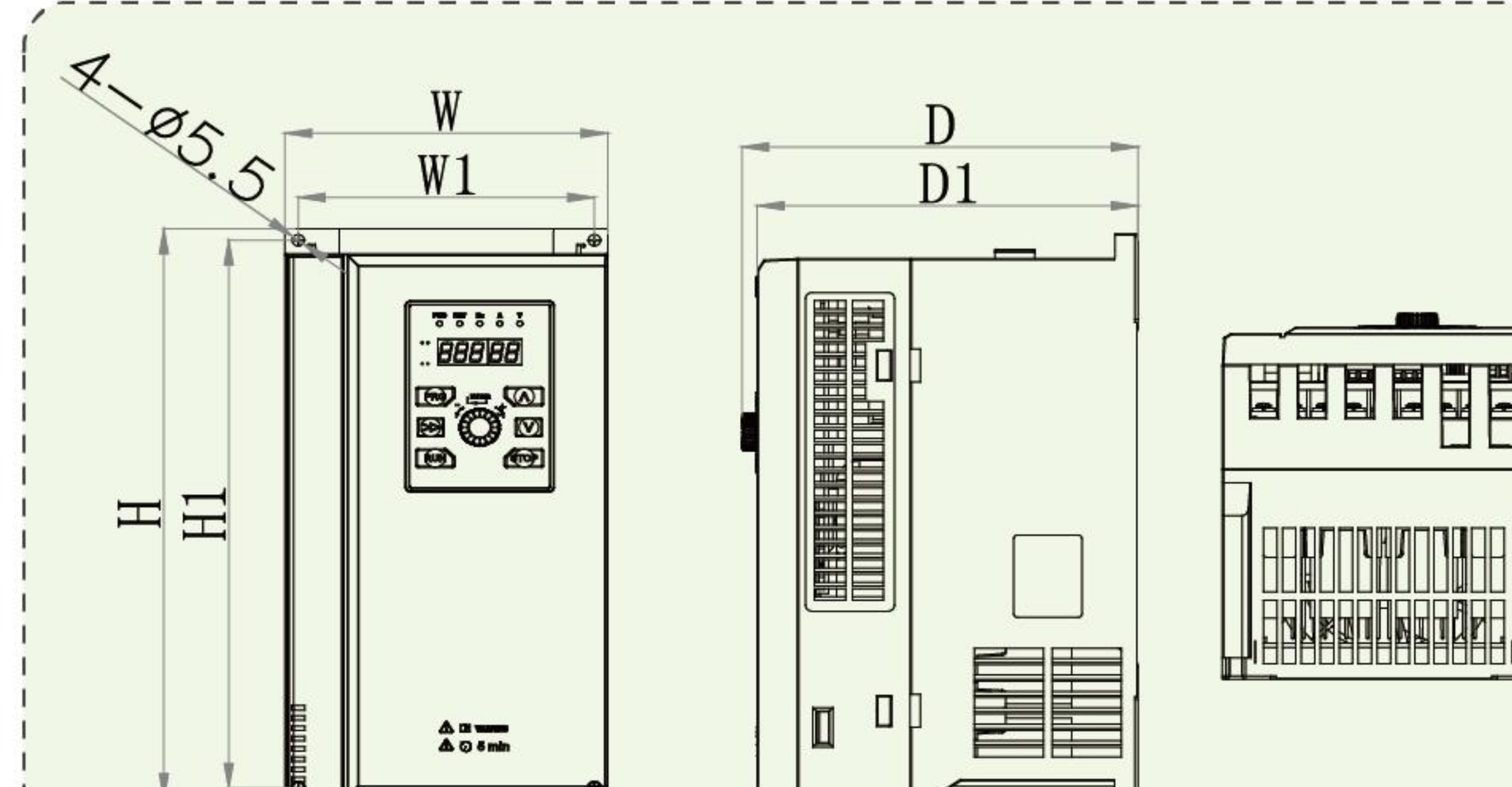
(c)规格尺寸
