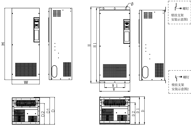
(c) C 规格尺寸
