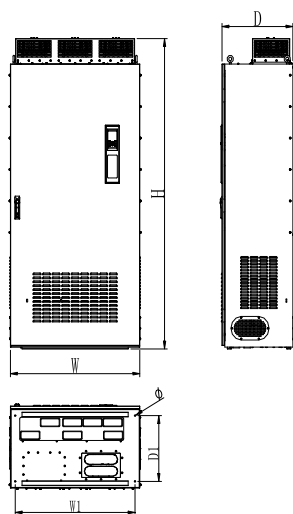
(c) C 规格尺寸
